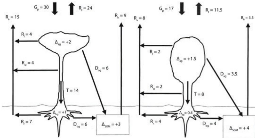
Figure 2: Estimated Annual Total C Flows in Tonne/ha/yr in (a) a Tropical Rainforest (Amazonia) and (b) a Temperate Deciduous Oak-hickory Forest (Tennessee, US)
